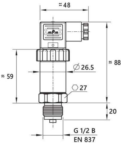
Angular Connector form A
