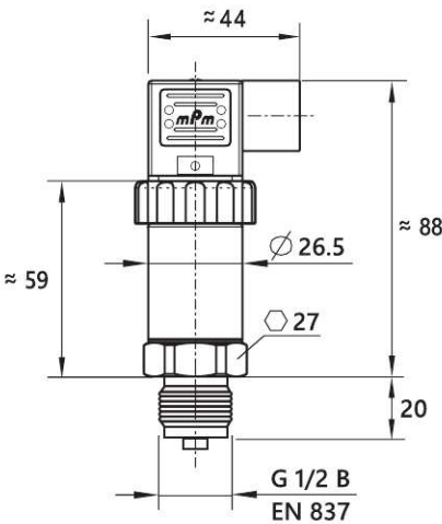
Angular Connector form C
